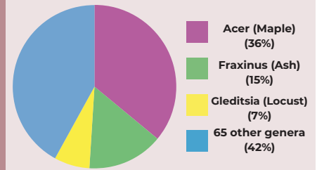
Genus Diversity
