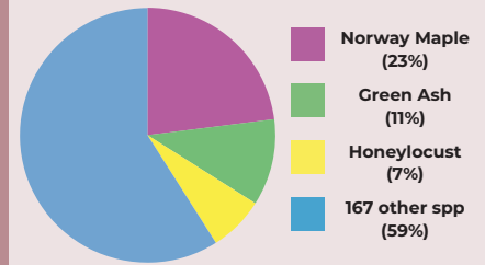
Species Diversity
